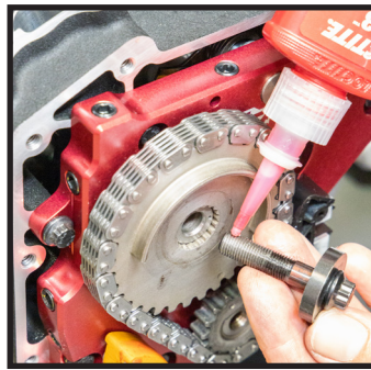
Press front cam into ball bearing, rear cam slip fits into roller bearing.
