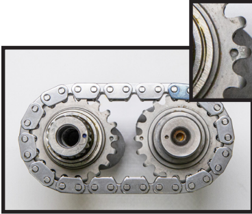
Install chain on the cams & verify that the timing marks are aligned.
