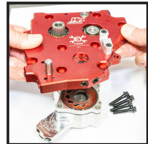
Attach oil pump to the camplate finger tight.
